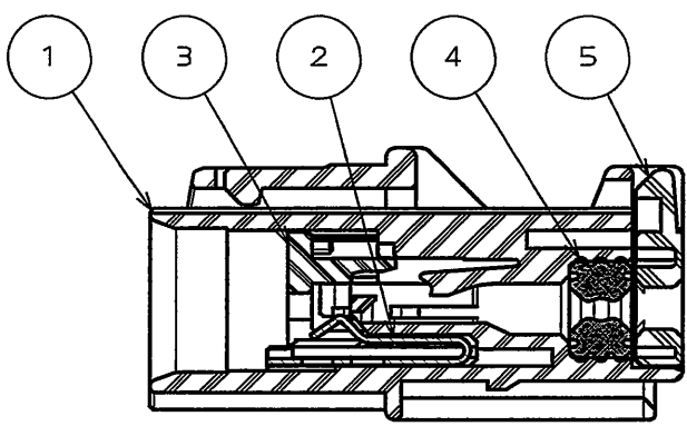
SECT. A-A
