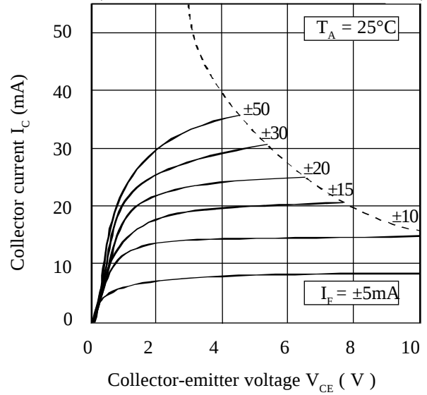
Collector Current vs. Collector-emitter Voltage ( normalized to SFH620-2 & SFH620-3 )
