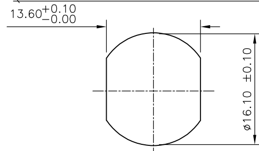
RECOMMENDED PANEL CUT-OUT (MAX PANEL THICKNESS 4.5mm)
