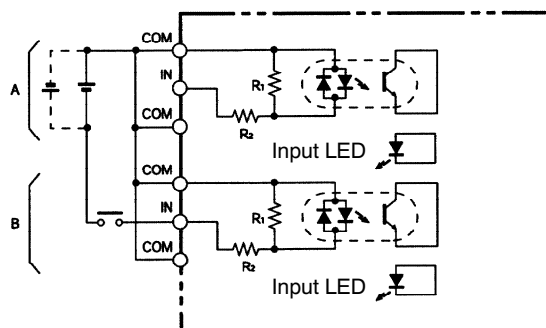
CQM1-ID112/213/214
