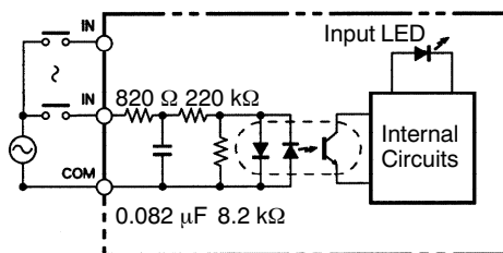
CQM1-IA221
