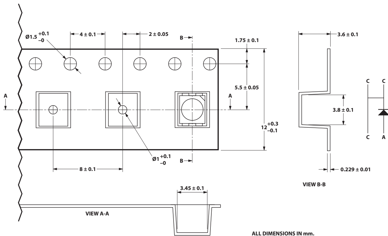
Figure 13. Tape dimensions
