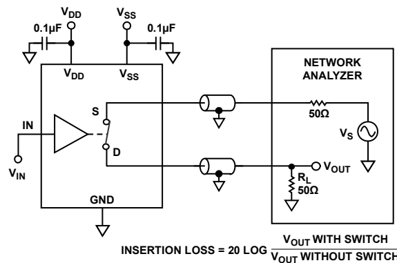
Figure 24. Bandwidth
