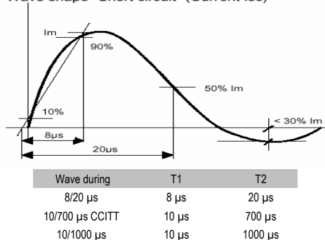
Wave shape "Short circuit" (Current Isc)
