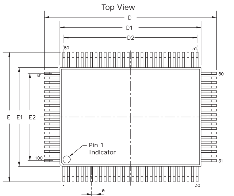
Figure 11. Package Drawing
