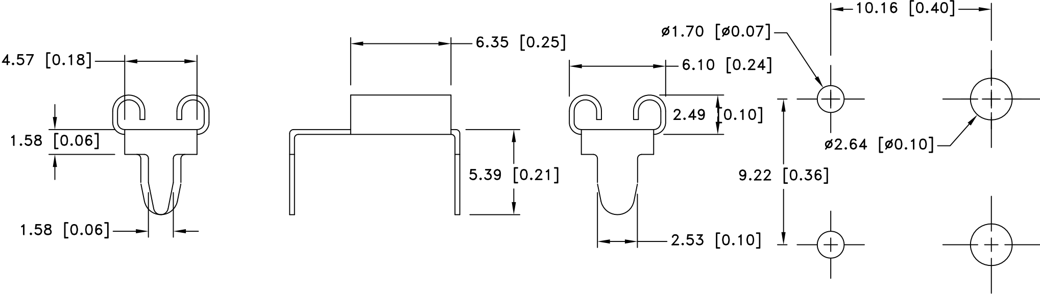
MOUNTING DETAIL FOR TWO CLIPS
