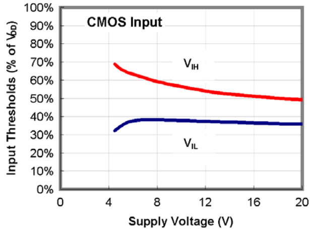
Figure 24. Input Threshold % vs. Supply Voltage
