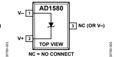
Figure 2. SC70
