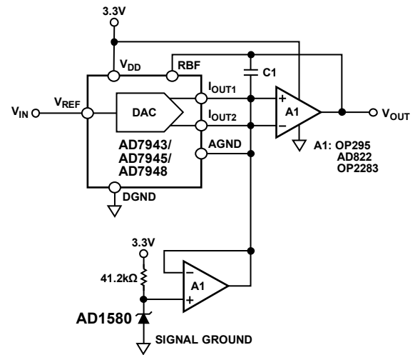
Figure 26. Single-Supply System
