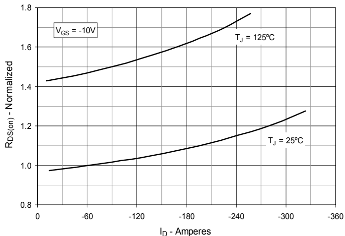
Fig. 5. R_{DS(on)} Normalized to I_D = -60\text{A} vs. Drain Current
