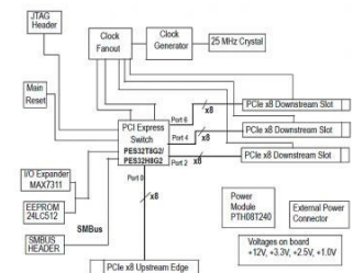
89KTPES32T8G2 Eval Board Functional Diagram
