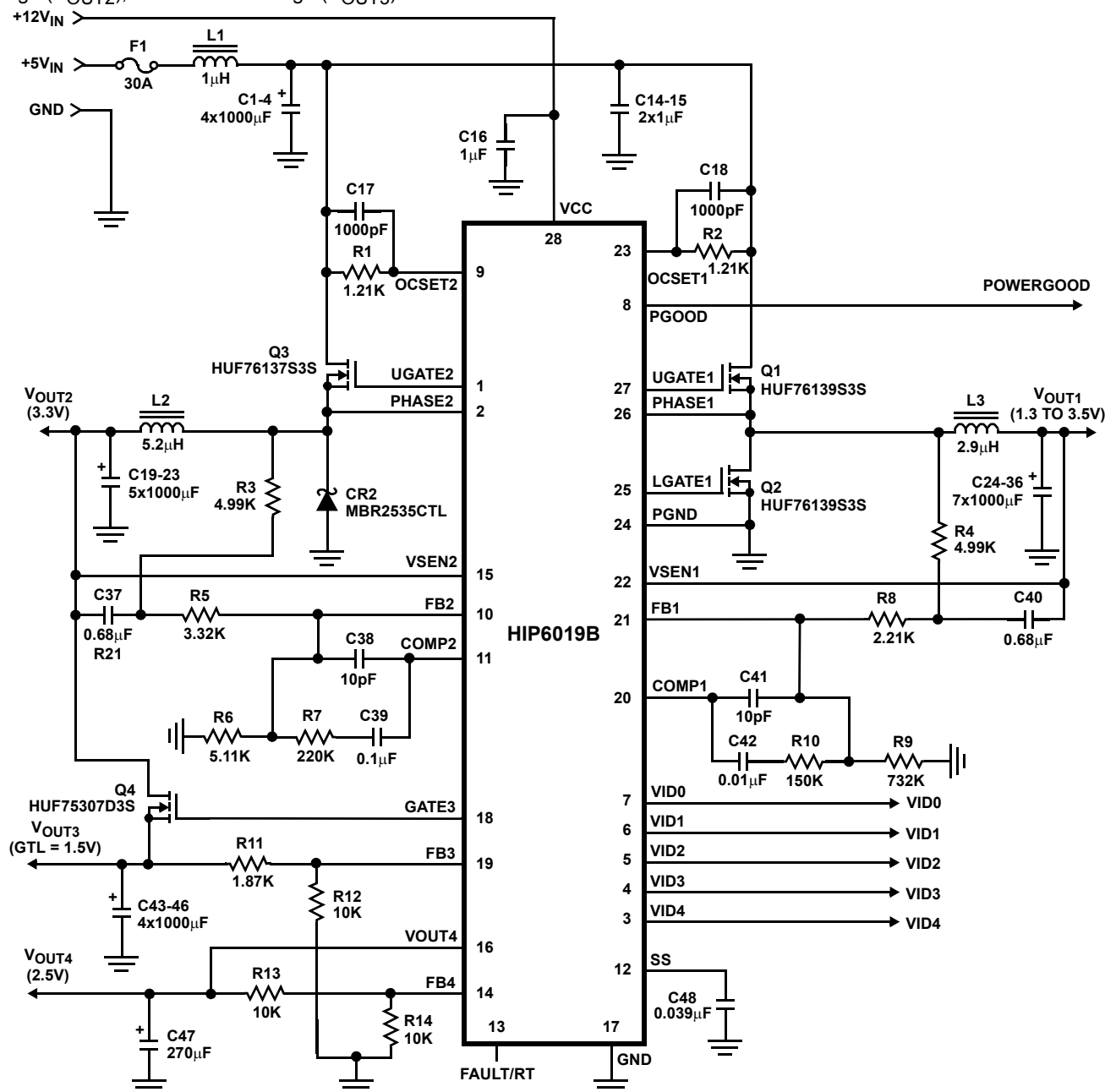
FIGURE 15. APPLICATION CIRCUIT
