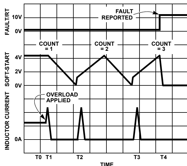
FIGURE 8. OVER-CURRENT OPERATION
