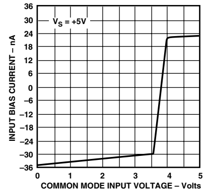
TPC 24. Input Bias Current vs. Common-Mode Voltage, V_S = +5\text{ V}
