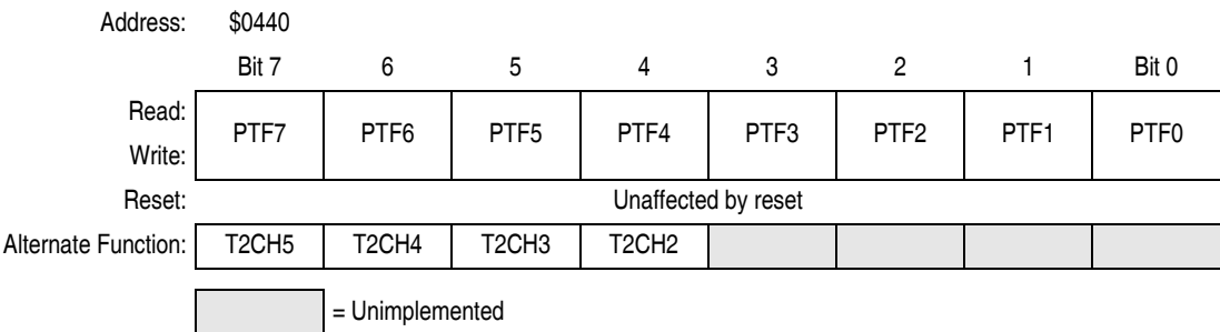
Figure 12-20. Port F Data Register (PTF)
