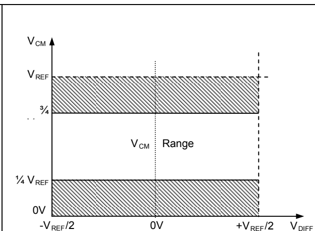
Figure 7: Input voltage range for bipolar mode
