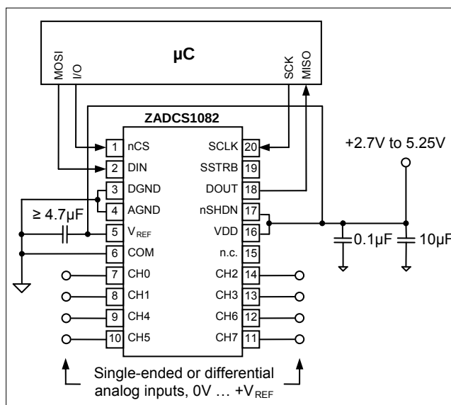
Figure 5: Basic application schematic for ZADCS1082
