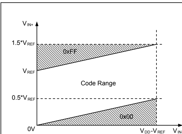
Figure 6: Input voltage range in unipolar mode
