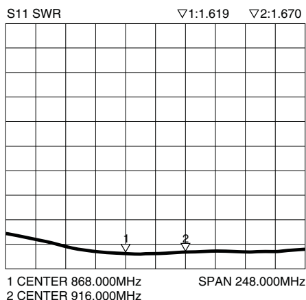
Typical VSWR
