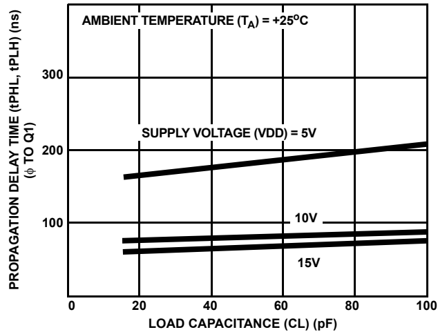
FIGURE 9. TYPICAL PROPAGATION DELAY TIME AS A FUNCTION OF LOAD CAPACITANCE (φ TO Q1)
