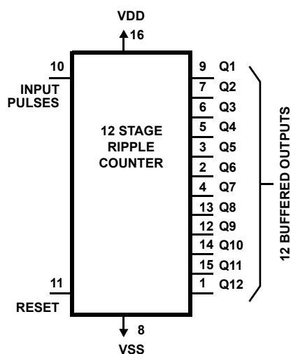
CD4040BMS
