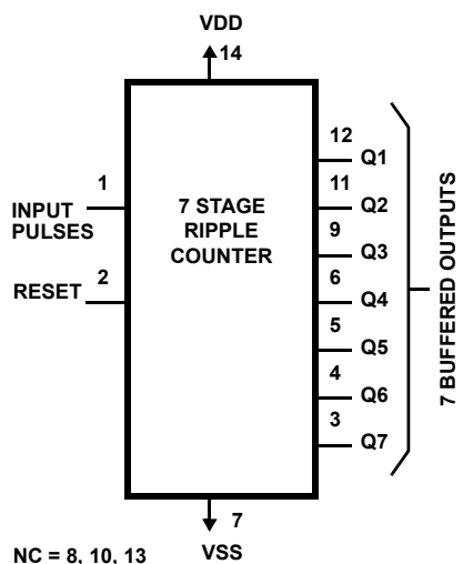
CD4024BMS
