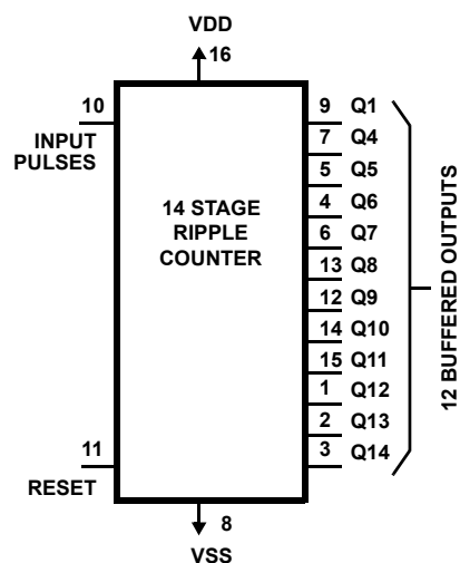
CD4020BMS
