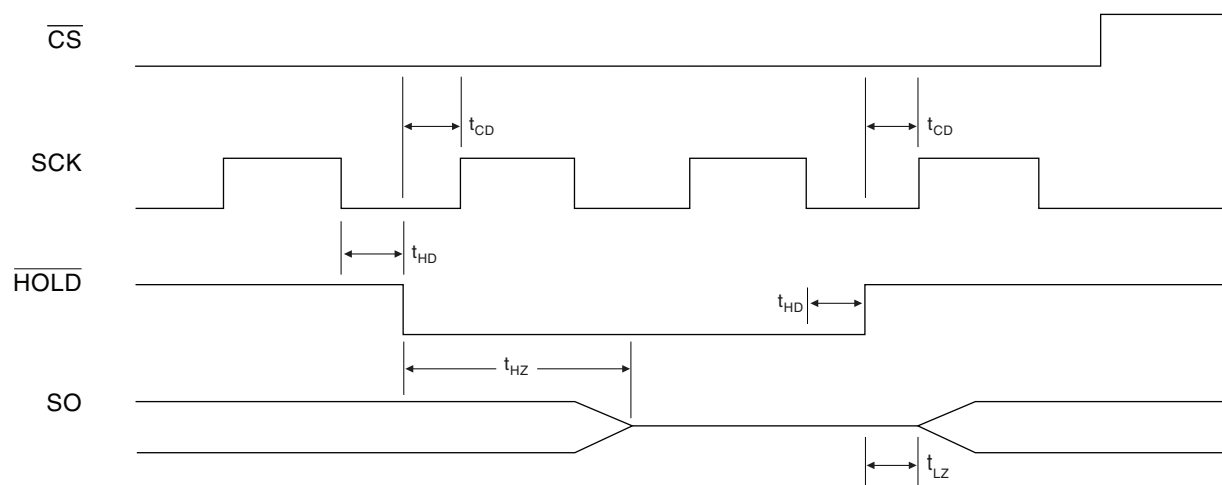
Figure 5-8. \overline{\text{HOLD}} Timing
