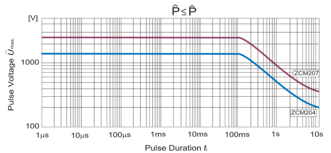
Pulse Voltage
