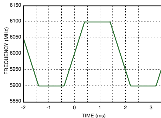
Frequency Sweep
