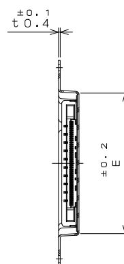
SECT. C-C 断面C-C (SCALE 1:1)
