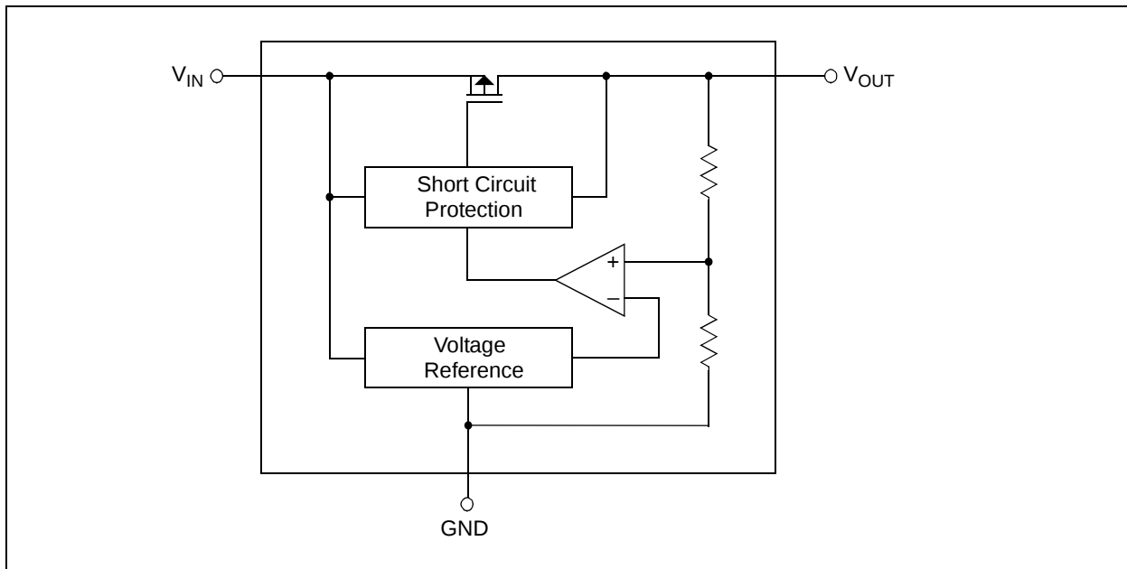
FIGURE 4-1: Block Diagram.
