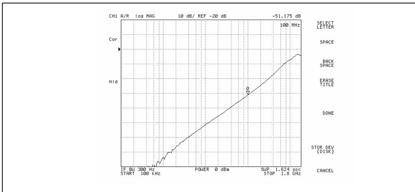
Fig 3. Crosstalk
