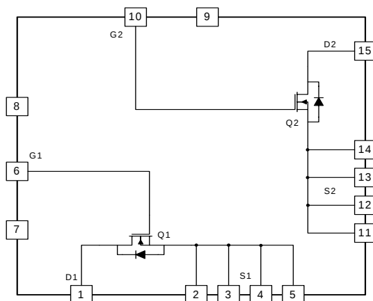
Figure 1. FD6M045N06 Module Block Diagram
