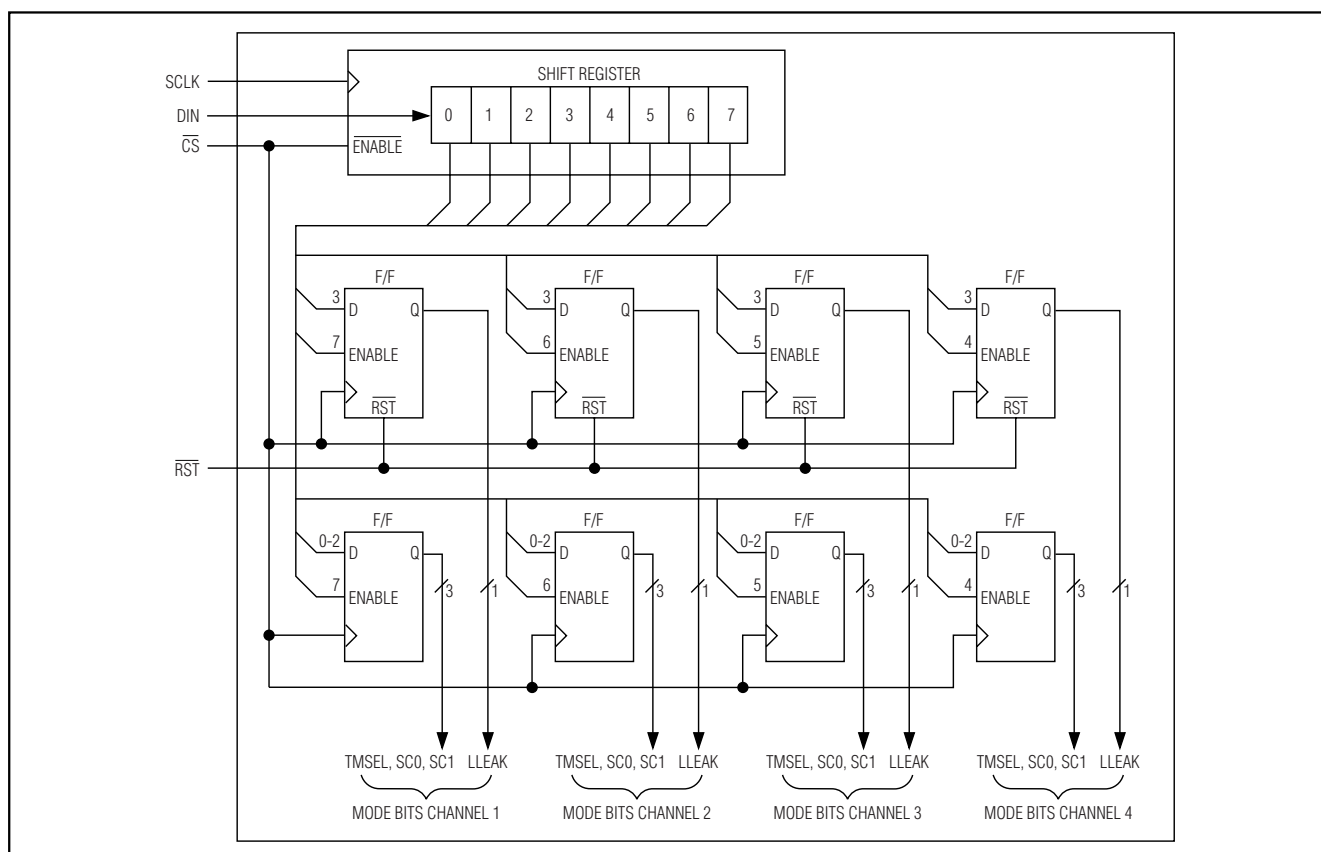
Figure 6. Serial Interface
