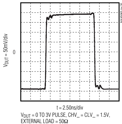
COMPARATOR DIFFERENTIAL OUTPUT RESPONSE (MAX996_ _GCCQ)
