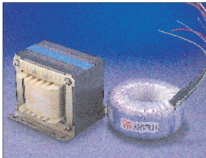
Overall Comparison of 250 VA E-I-Core AMVECO Isolation Transformer vs. 250 VA E-I Core Isolation Transformer
