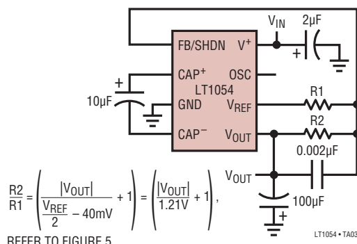
Basic Voltage Inverter/Regulator
