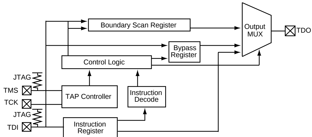
Figure 1-12 • 42MX IEEE 1149.1 Boundary Scan Circuitry
