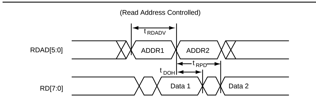
Figure 1-29 • 42MX SRAM Asynchronous Read Operation—Type 1
