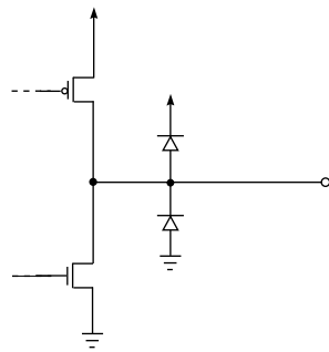
Figure 3-7: Indicator Outputs: \overline{SD}/\overline{HD} , LOCKED, LOS
