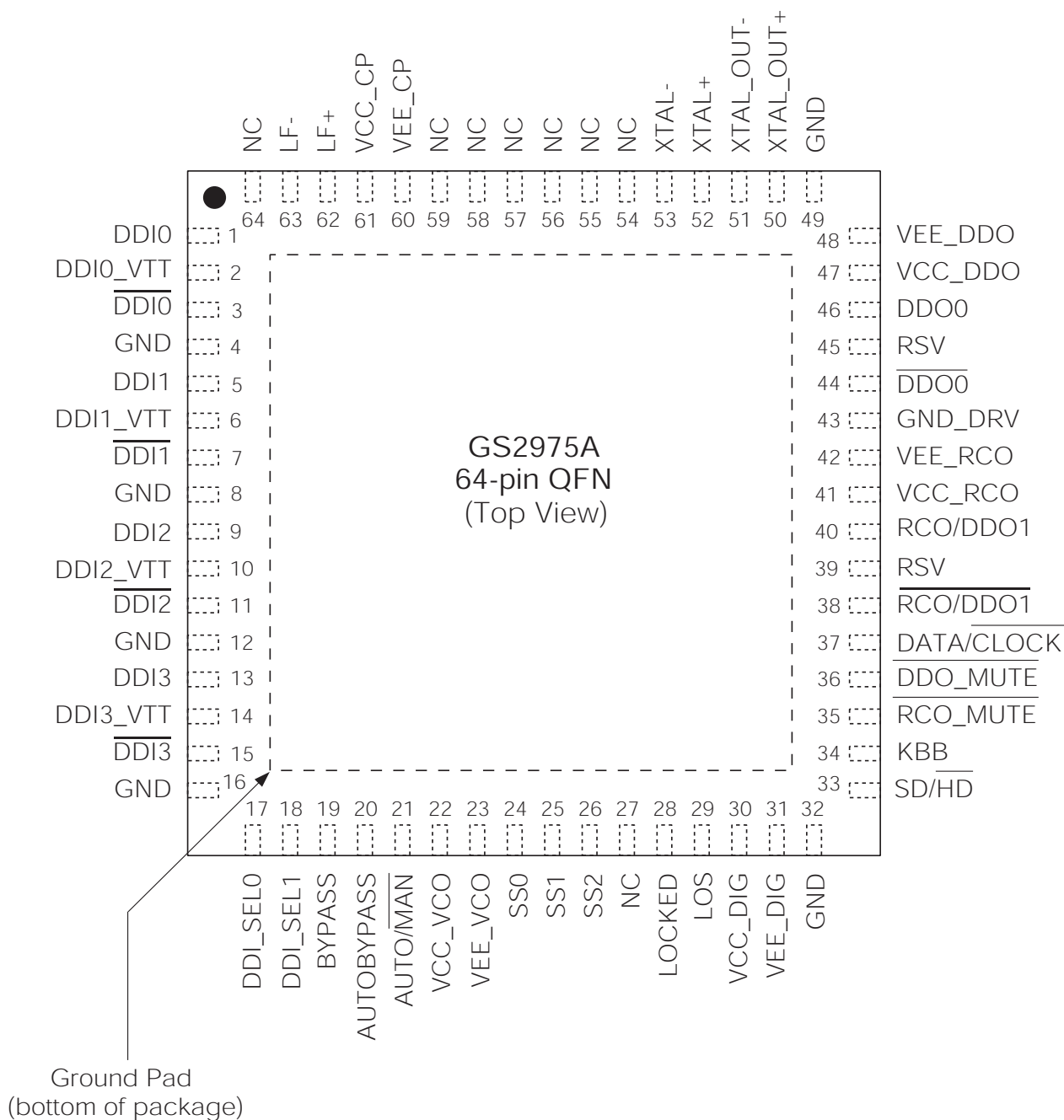
Figure 1-1: 64-Pin QFN
