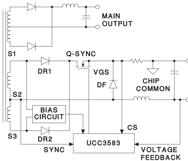
Figure 3. Half-bridge synchronous post regulator application.
