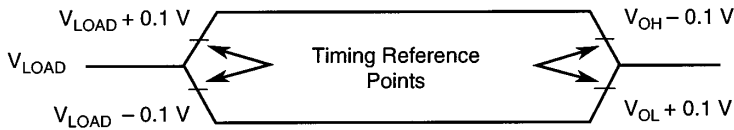
Figure 15. Float Waveforms
