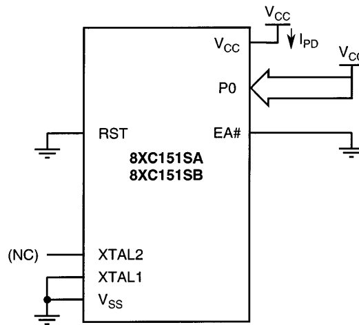
Figure 5. I_{PD} Test Condition, Powerdown Mode, V_{CC} = 2.0V - 5.5V
