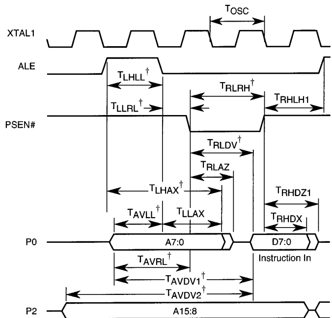
Figure 7. External Instruction Bus Cycle in Nonpage Mode
