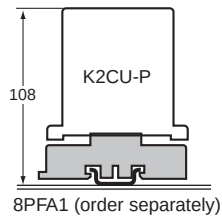
Connecting Socket
