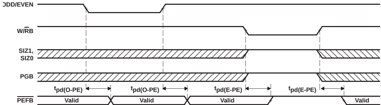
Figure 16. ODD/EVEN, W/RB, SIZ1, SIZ0, and PGB to PEFB
