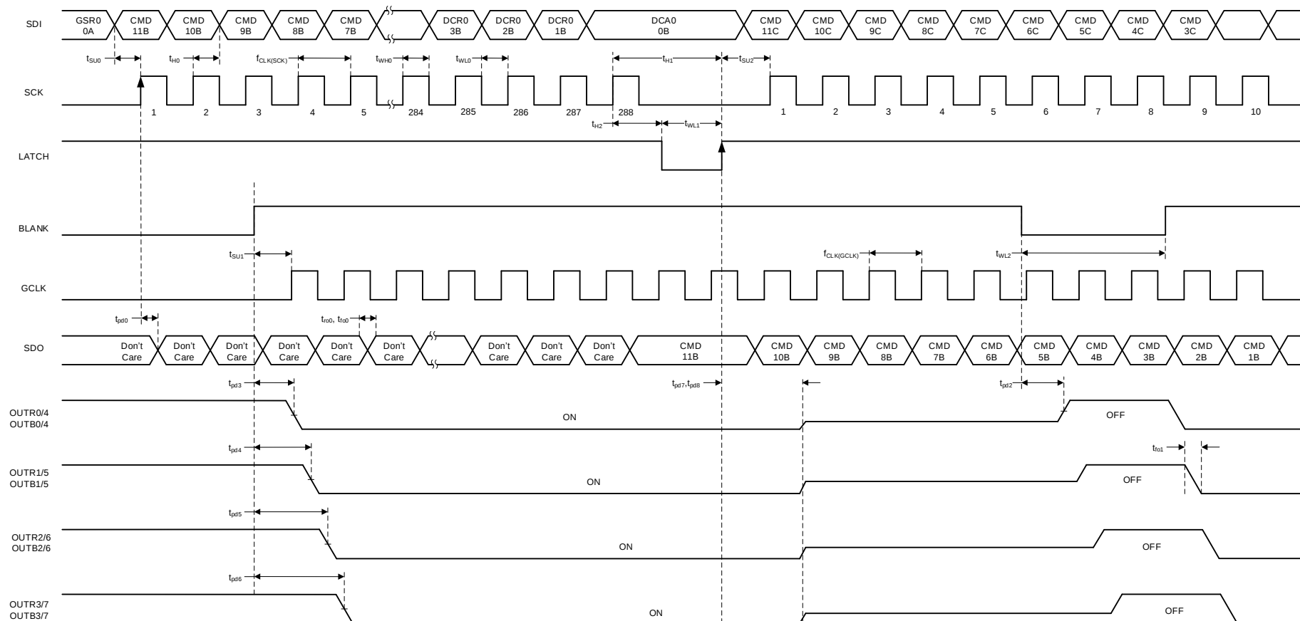
Figure 2. Function-Control, Brightness-Control, and Dot-Correction (FC-BC-DC) Data Write
