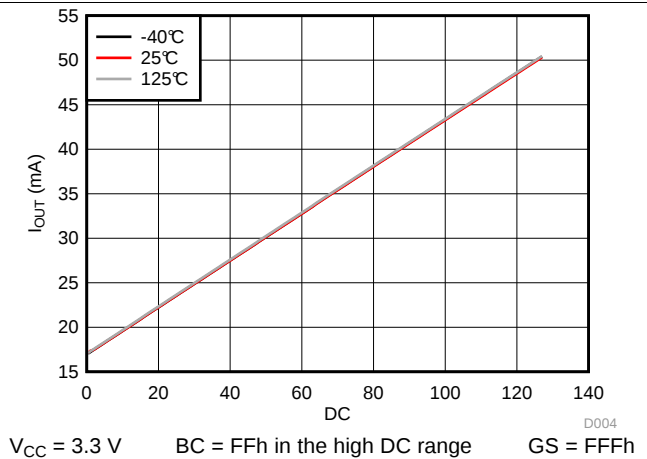
Figure 18. I_{OUT} vs Dot Correction at Different Ambient Temperatures
