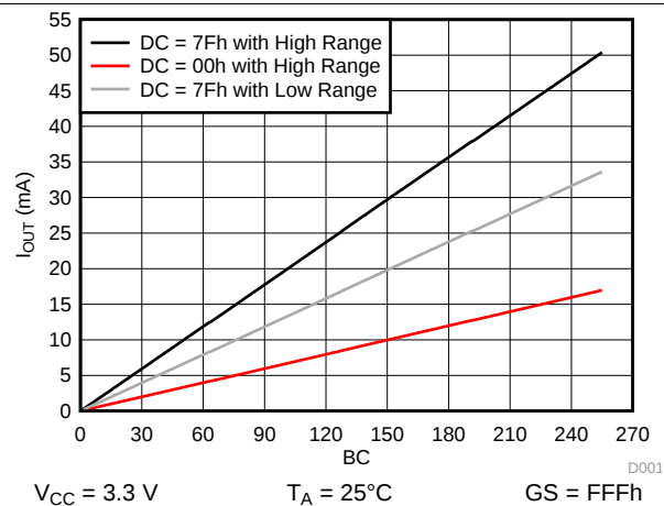
Figure 19. I_{OUT} vs Brightness Control in Different DC Ranges
