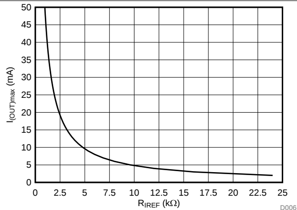
Figure 15. I_{OUTmax} vs R_{REF}
