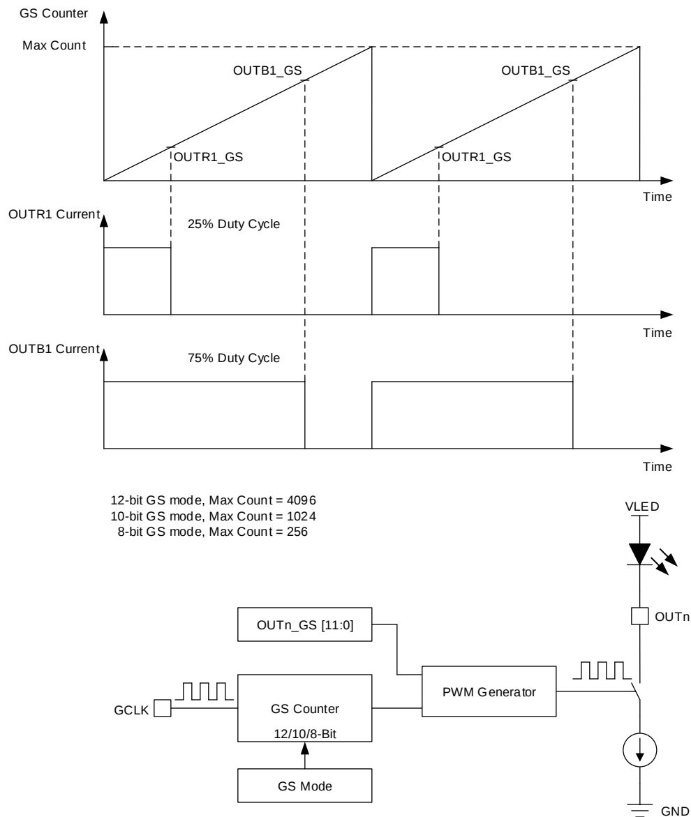
Figure 22. PWM Generator
