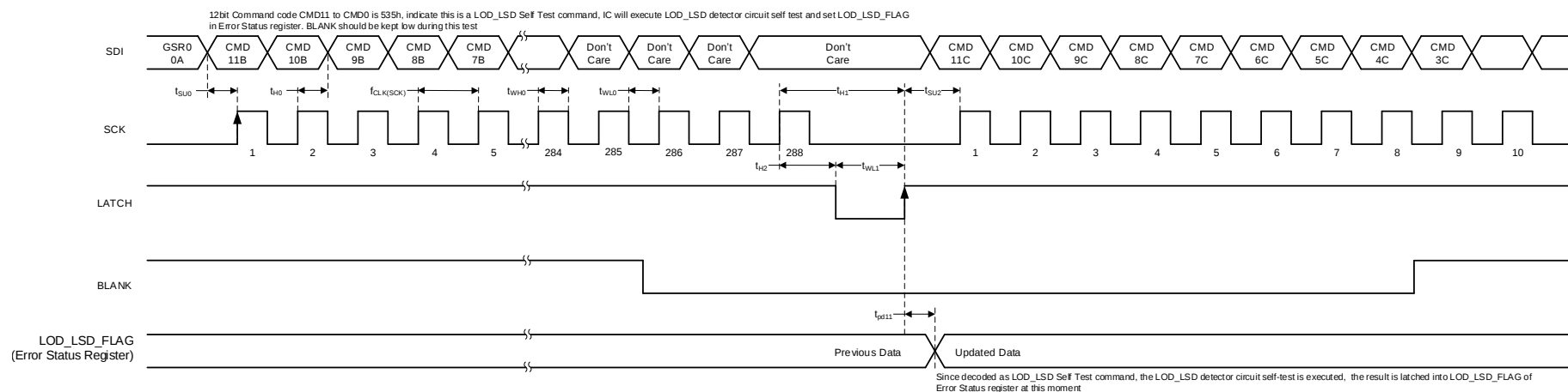
Figure 7. LOD_LSD Self-Test
