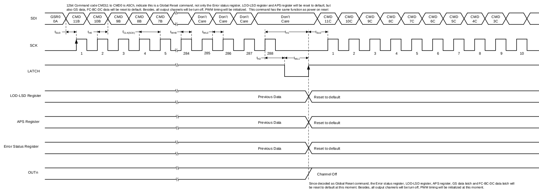
Figure 10. Global Reset
