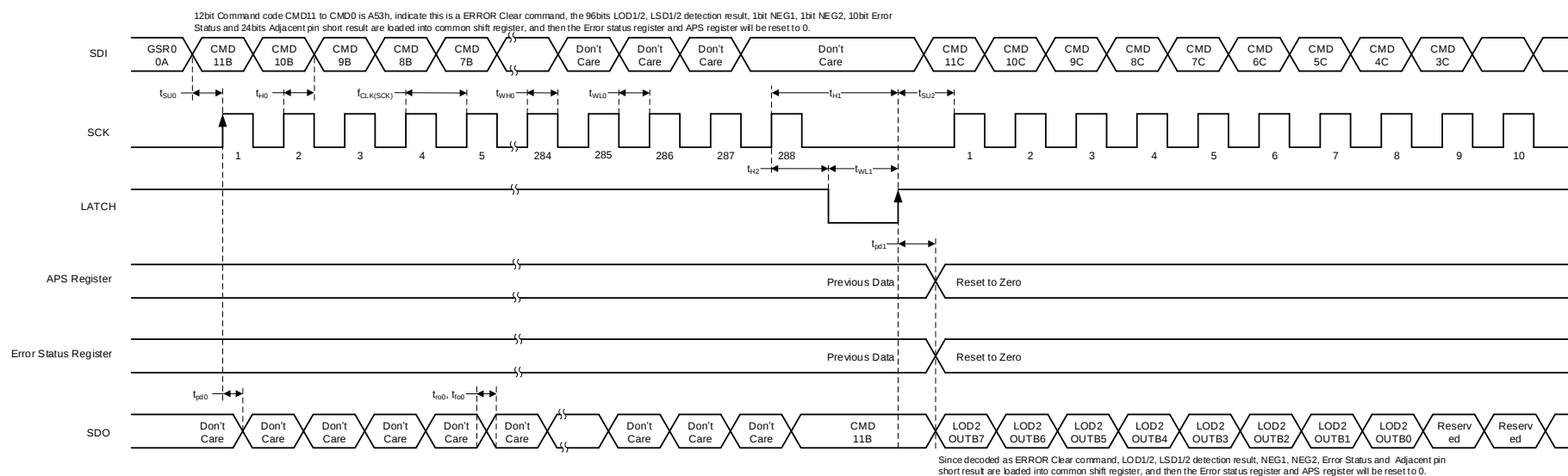
Figure 9. ERROR Clear
