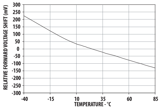
Figure 14. Temperature vs. relative forward voltage shift
