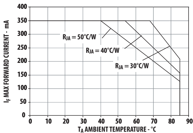
Figure 11. Maximum forward current vs. ambient temperature for InGaN Derated based on T_{JMAX} = 110^{\circ}\text{C} , R_{\theta JA} = 30^{\circ}\text{C/W} / 40^{\circ}\text{C/W} and 50^{\circ}\text{C/W}
