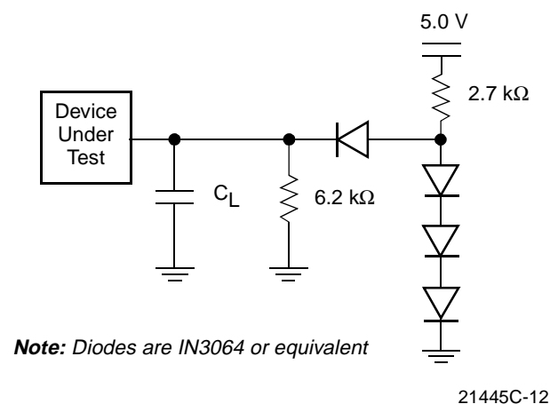
Figure 7. Test Setup
