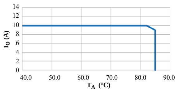
BR200, V_{OUT} = 1.5\text{ V} , V_{IN} = 12\text{ V} 1.5 m/s Airflow
