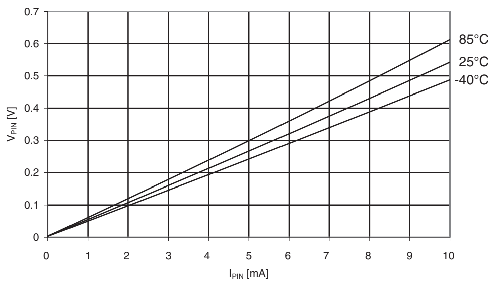
Figure 33-68. I/O pin output voltage vs. sink current. V_{CC} = 3.3V .
