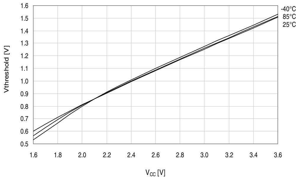
Figure 33-179. I/O pin input threshold voltage vs. V_{CC} . V_{IL} I/O pin read as "0".
