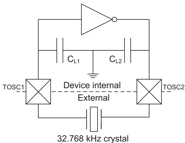
Figure 32-18.TOSC input capacitance.
