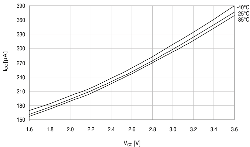
Figure 33-163. Idle mode supply current vs. V_{CC} . f_{SYS} = 2\text{MHz} internal oscillator.
