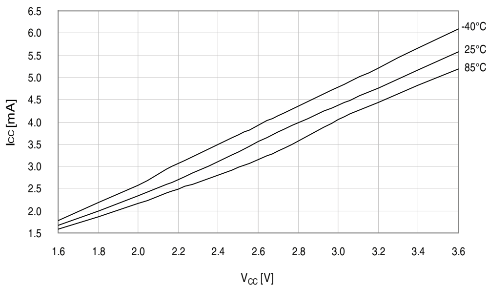
Figure 33-291. Active mode supply current vs. V_{CC} . f_{SYS} = 32\text{MHz} internal oscillator prescaled to 8MHz.
