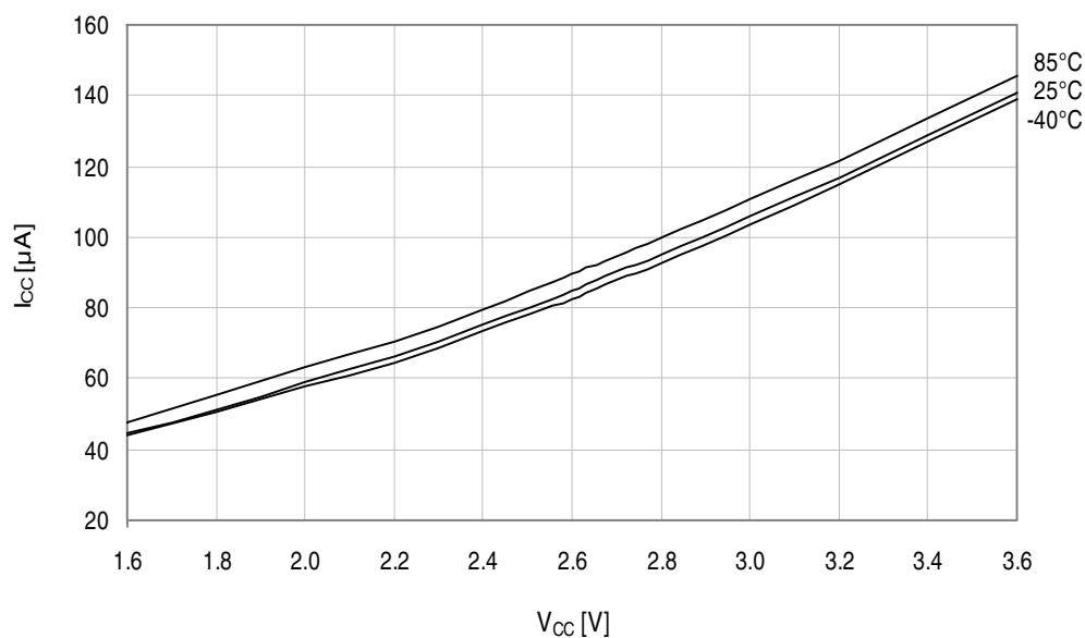
Figure 33-162. Idle mode supply current vs. V_{CC} . f_{SYS} = 1\text{MHz} external clock.
