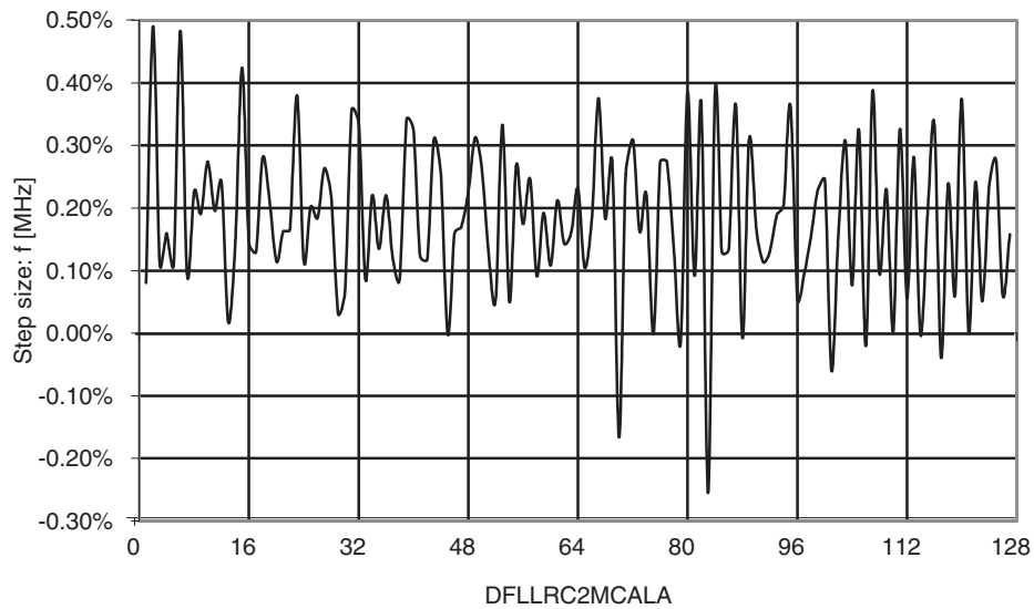
Figure 33-77. Internal 2MHz oscillator CALA calibration step size.
