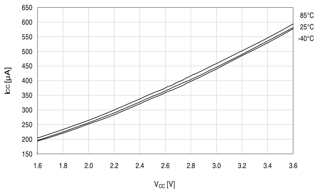
Figure 33-290. Active mode supply current vs. V_{CC} . f_{SYS} = 2\text{MHz} internal oscillator.
