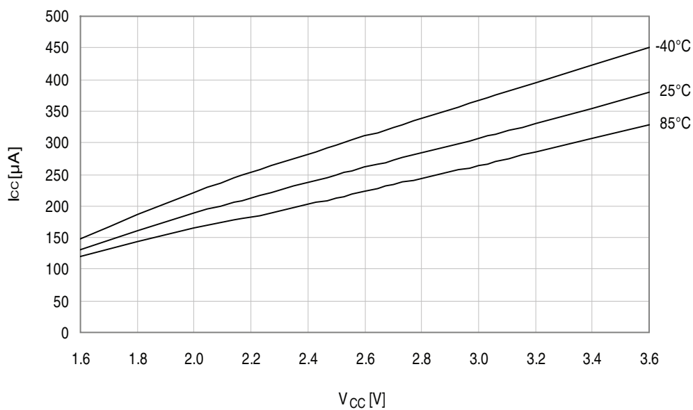
Figure 33-288. Active mode supply current vs. V_{CC} . f_{SYS} = 32.768\text{kHz} internal oscillator.
