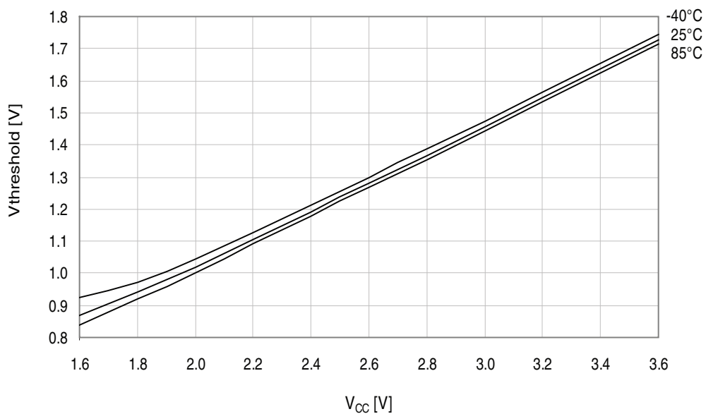
Figure 33-178. I/O pin input threshold voltage vs. V_{CC} . V_{IH} I/O pin read as "1".
