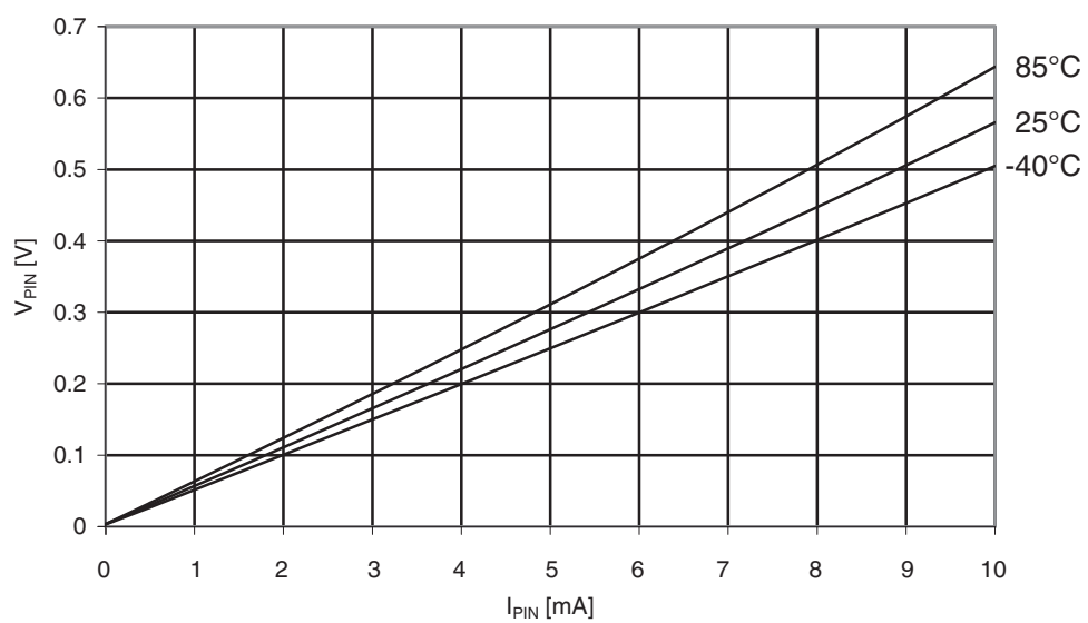
Figure 33-67. I/O pin output voltage vs. sink current. V_{CC} = 3.0V .
