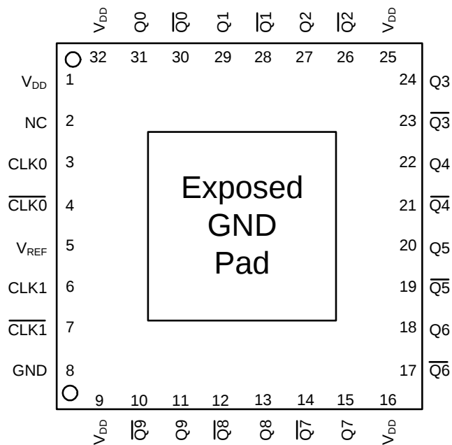
Figure 9. 32-QFN Pin Diagram
