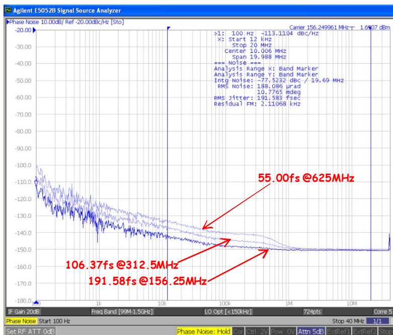
Total Jitter
