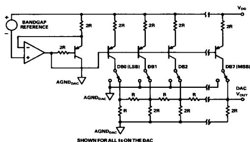
Figure 3. DAC Simplified Circuit Diagram
