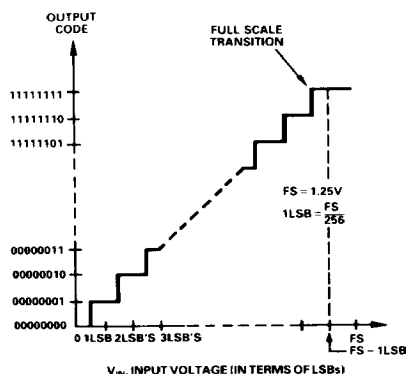
Figure 22. Nominal Transfer Characteristic for Unipolar (0 to +1.25V) Operation
