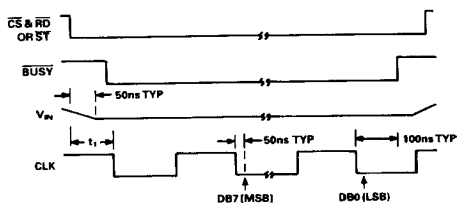
Figure 4. Operating Waveforms Using External Clock
