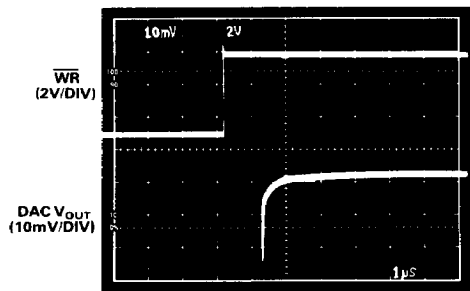
Positive-Going Settling Time ( \pm 2.5V Range)
