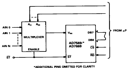
Figure 11. Multichannel Inputs
