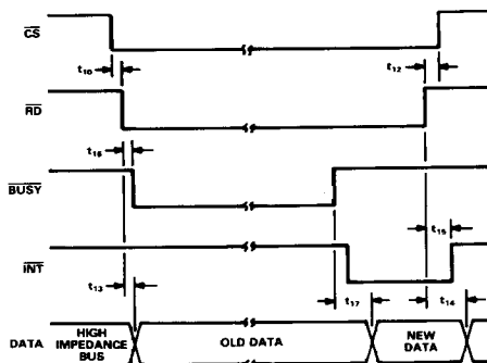
Figure 12. ADC Mode 2 Interface Timing
