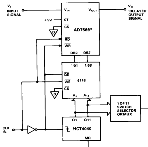
Figure 28. Analog Delay Line
