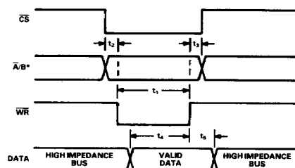
Figure 7. AD7569 DAC Input Control Logic
