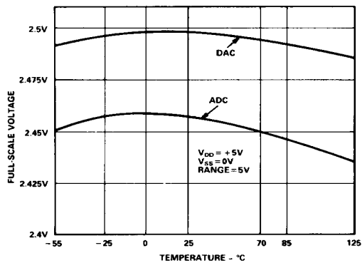
DAC/ADC Full-Scale Temperature Coefficient
