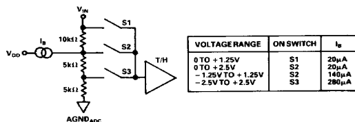
Figure 5. Equivalent V_{IN} Circuit
