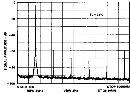
Figure 15. DAC Output Spectrum
