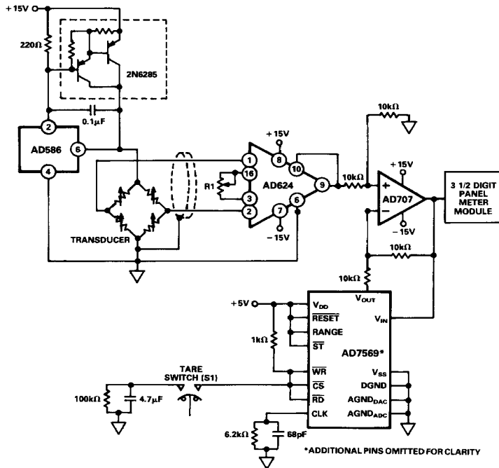
Figure 30. Weigh Scale System with Tare Function
