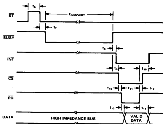
Figure 10. ADC Mode 1 Interface Timing
