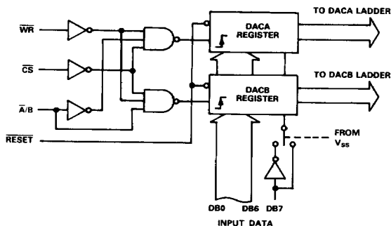
Figure 9. AD7669 DAC Control Logic
