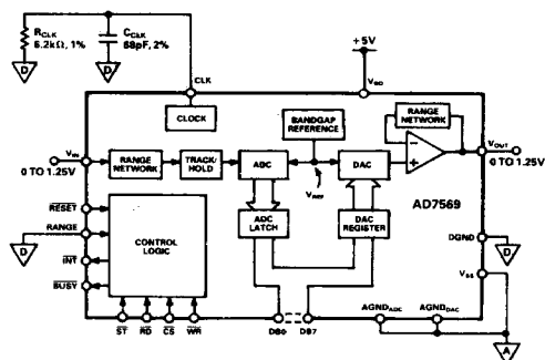
Figure 21. AD7569 Unipolar (0 to +1.25V) Operation
