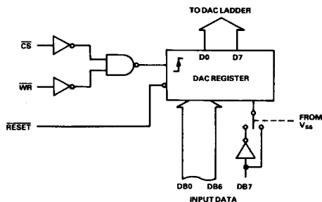
Figure 7. AD7569 DAC Input Control Logic
