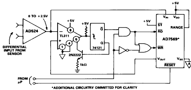
Figure 25. Peak-Reading A/D Converter
