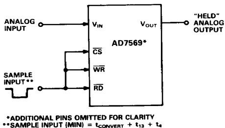
Figure 29. Infinite Sample-and-Hold
