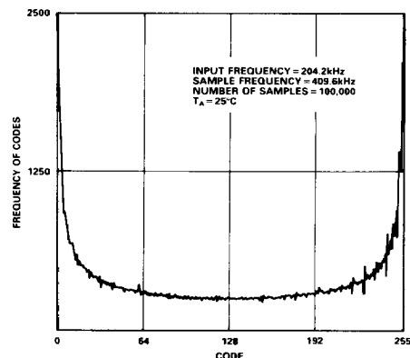
Figure 16. ADC Histogram Plot
