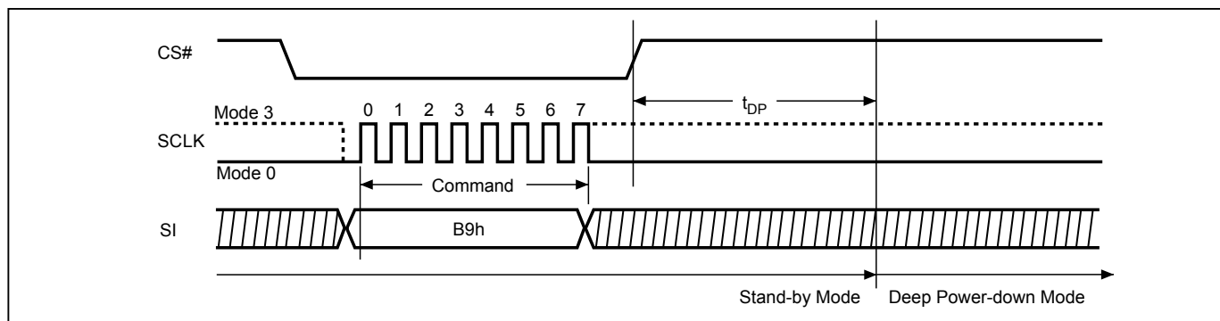
Figure 47. Deep Power-down (DP) Sequence (SPI Mode)
