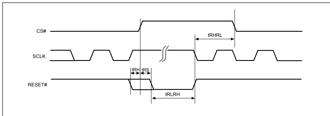
Figure 59. RESET Timing
