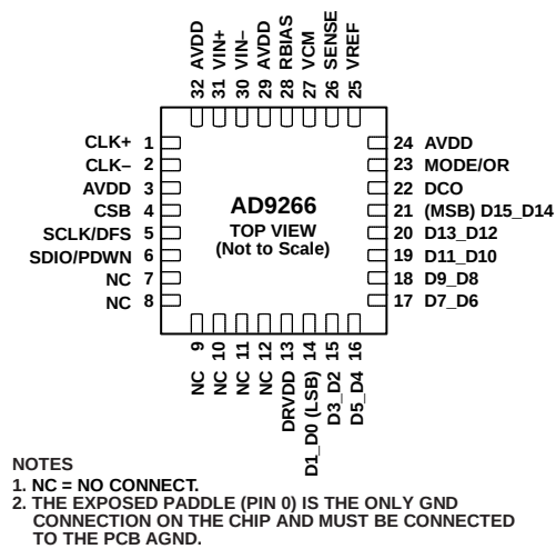
Figure 3. Pin Configuration
