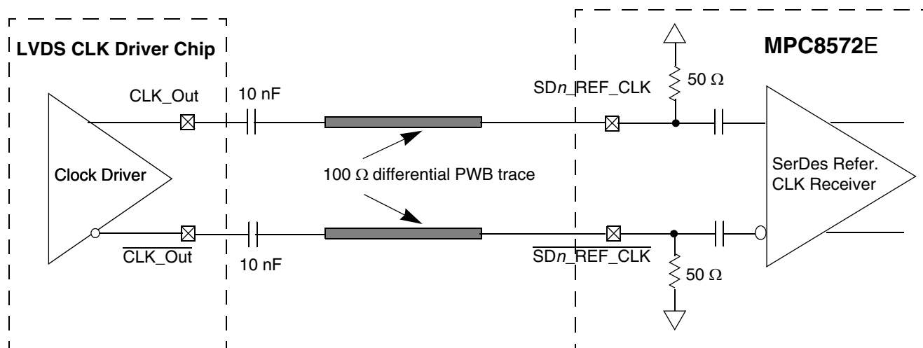
Figure 49. AC-Coupled Differential Connection with LVDS Clock Driver (Reference Only)
