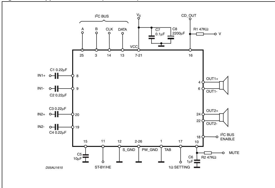
Figure 24. Application circuit (TDA7575B)
