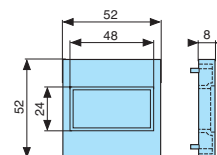
Accessory 26 546 830
