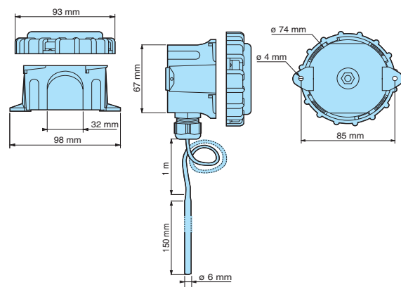
89 750 153 and 89 750 155
