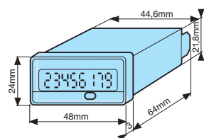
Unit spacing
