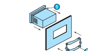
Accessory 2108 - 2108H 26 546 831
