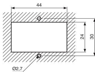
99 766 7 : Panel cut-out
