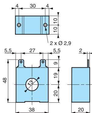
Current transformer
