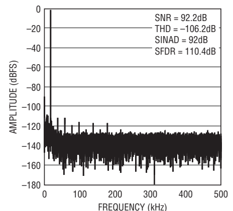
32k Point FFT f_S = 1 Msps, f_{IN} = 20 kHz
