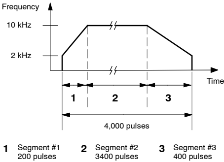
Figure 6-31 Frequency/Time Diagram
