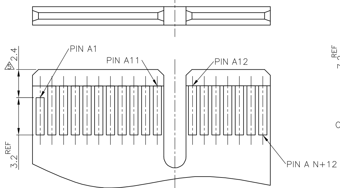
MODULE LAYOUT(MATING PART ONLY)
